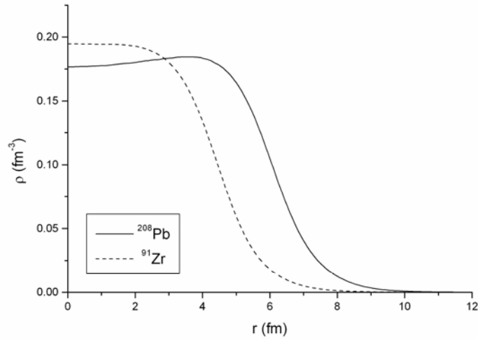
Figure 3 Nuclear density profiles at T = 0 MeV.
