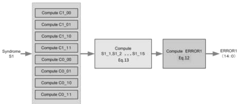
Figure 5 Block diagram of EP1.
