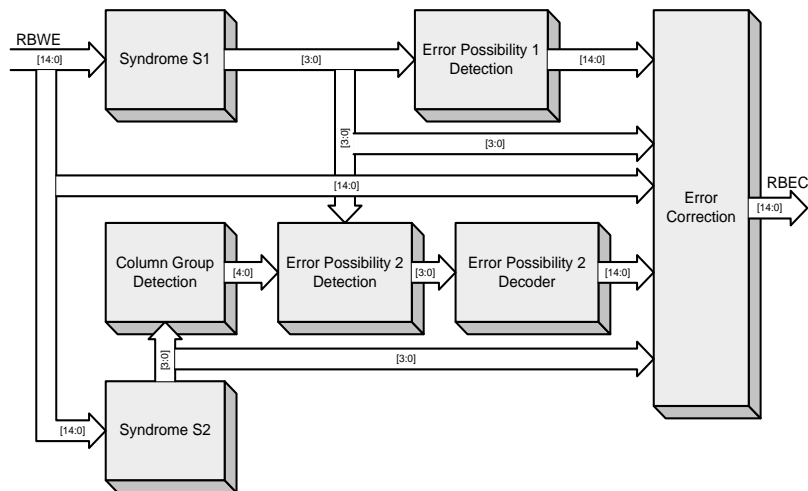
Figure 3 Block diagram of the BCH (15,7) decoder.
