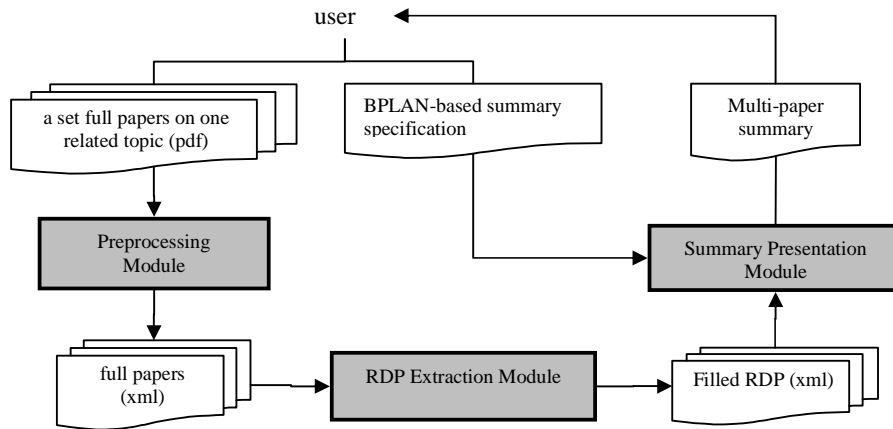
Figure 1 Diagram of tailored multi-paper summarization system architecture.
