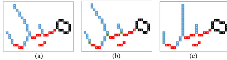
Figure 4 An Example of a Slant Correction Result of a Handwritten Arabic Text Image (ميل) After Completing the Second Part of the Proposed Method.
