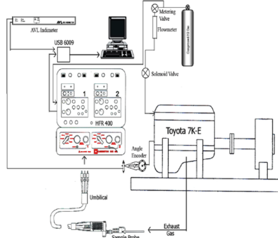
Figure 3. Scheme of experimental apparatus.
