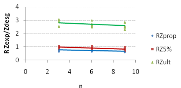
Figure 9. Ratio of experimental to design strength of senyon -plywood connection
