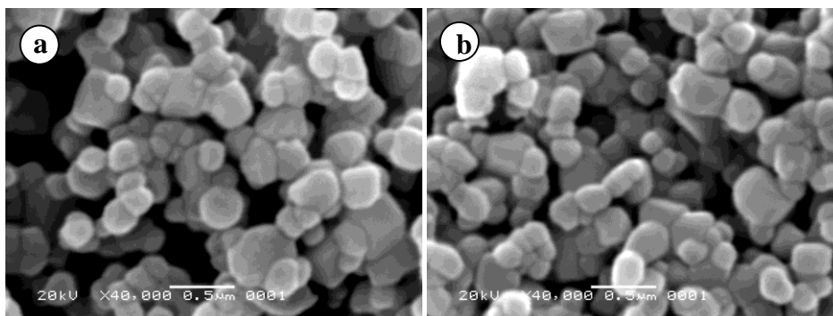
Figure 6 SEM images of filters at higher magnification: (a) prepared without addition of silica particles and (b) with addition of silica particles. The length of scale bar is 0.5 \mu\text{m} .
