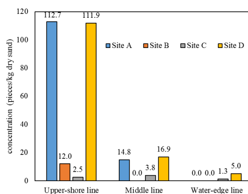
Figure 5 Concentration of microplastics at tide lines.
