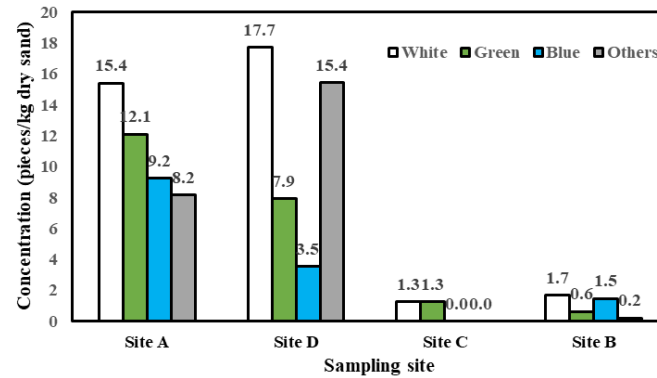
Figure 11 Distribution of microplastics by color.
