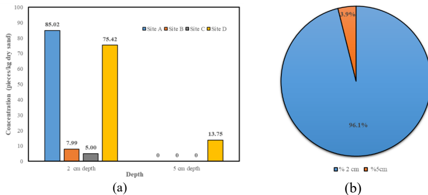
Figure 7 Concentration of microplastics by depth: (a) distribution of MPs by depth, (b) percentage of MPs at each depth.
