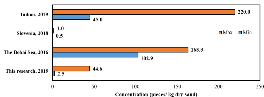
Figure 8 Comparison of the concentration of microplastics with other researches.
