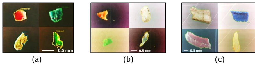
Figure 10 MPs of different sizes: (a) 0.5-1 mm, (b) 1-2.8 mm, (c) 2.8-5 mm. All scale bars are 0.5 millimeter.
