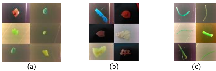
Figure 13 Different types of MPs: (a) granule, (b) fragments, (c) fibers.
