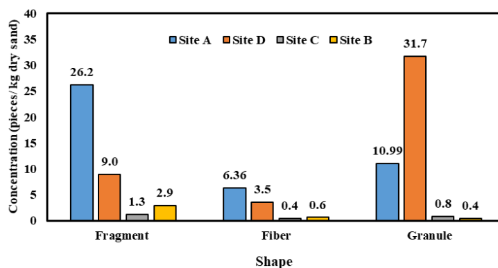
Figure 14 Concentration of microplastics by shape.
