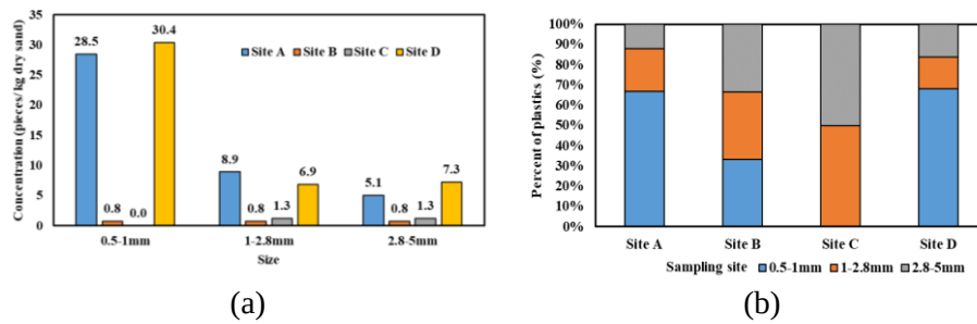
Figure 9 Distribution of microplastics by size: (a) concentration of MPs at each site, (b) percentage of MPs at each site.
