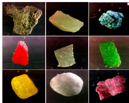
Figure 12 MPs in different colors.
