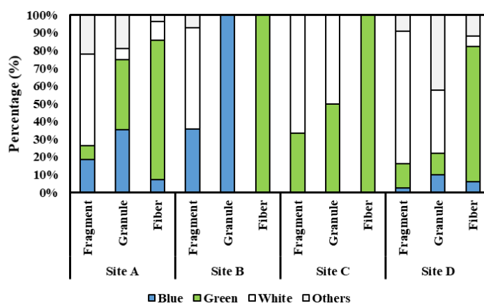
Figure 15 Distribution of shape by color.
