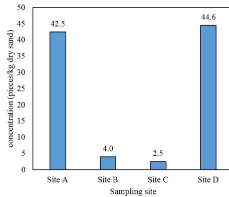
Figure 6 Average concentrations of microplastics.
