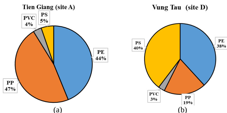
Figure 16 Concentration of microplastics by composition: (a) site A, (b) site D.
