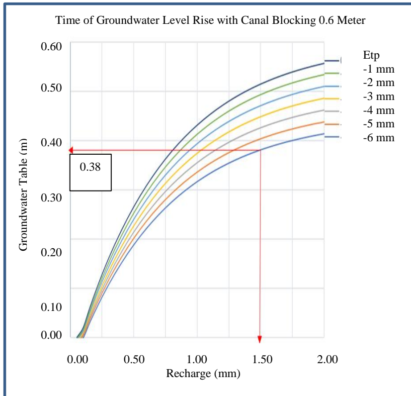
Figure 6 Time of rising groundwater chart.
