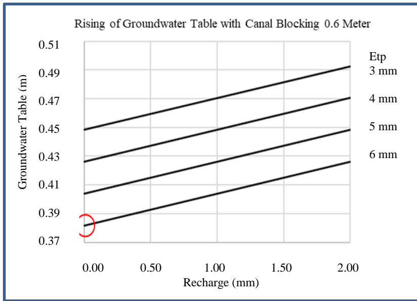
Figure 5 Rising groundwater graph.
