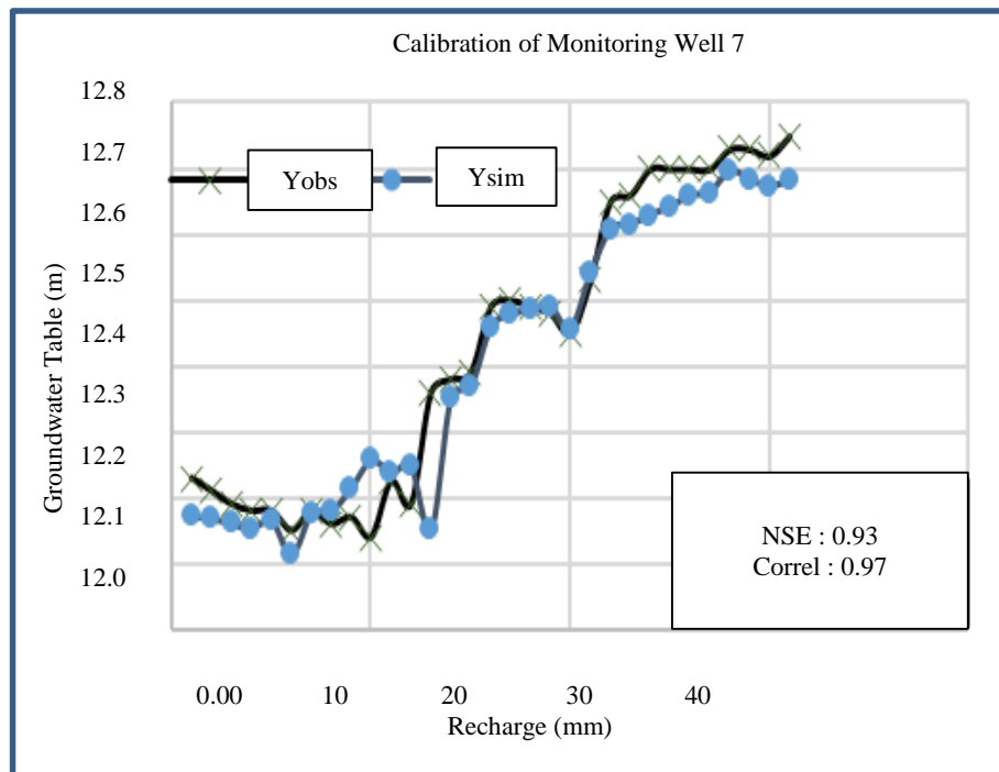
Figure 3 Calibration value (groundwater table from local level) [17].
