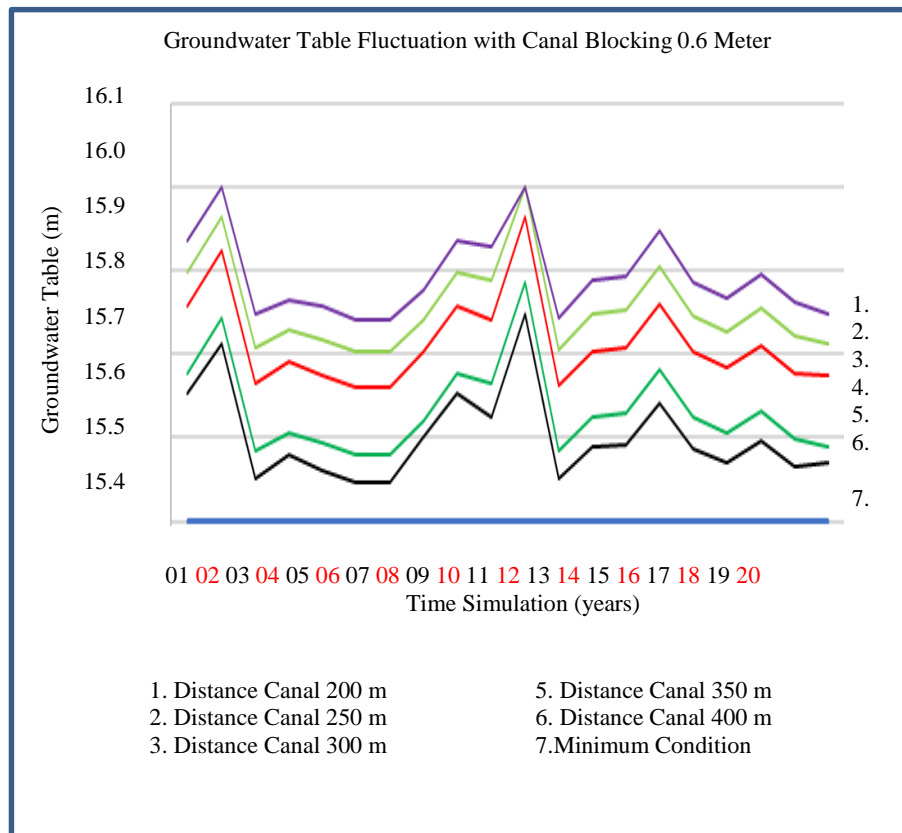
Figure 4 Fluctuation of the groundwater table, 1997-2016.
