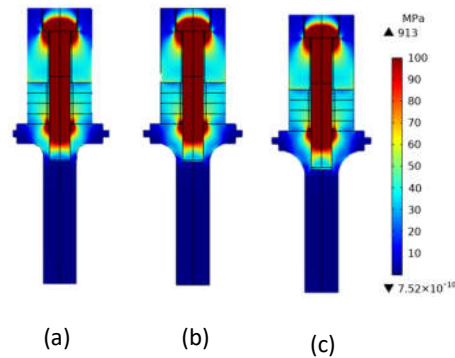
Figure 9 Simulation results of the stress distribution of the Model-3 transducer with a fillet radius of (a) 5 mm, (b) 7.5 mm, and (c) 10 mm on a bolt prestressed at 15 kN.
