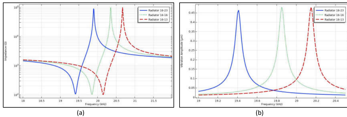
Figure 12 Simulation results of the Model-4 transducer (a) electrical impedance and (b) vibration amplitude with 16·23 mm (blue-solid), 16·16 mm (green dotted line), and 16·13 mm (red dash line) radiators for a 15 kN prestressed bolt.
