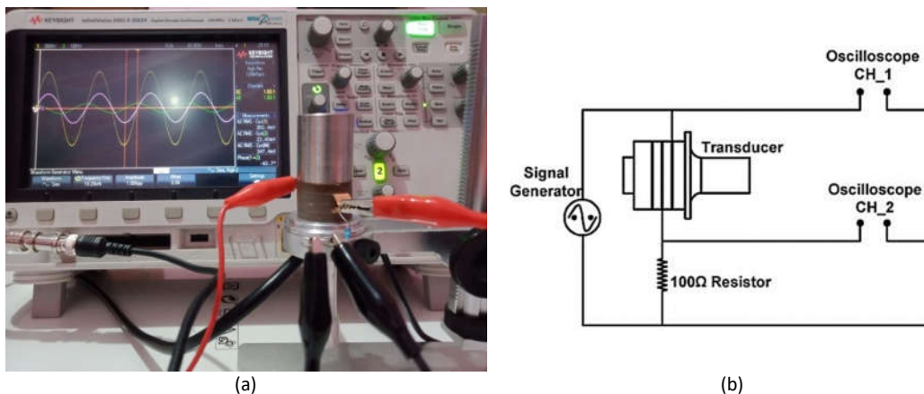
Figure 14 Setup for measuring transducer characteristics in the experiments: (a) actual measurements using an oscilloscope, and (b) scheme of the measurement set-up [11].
