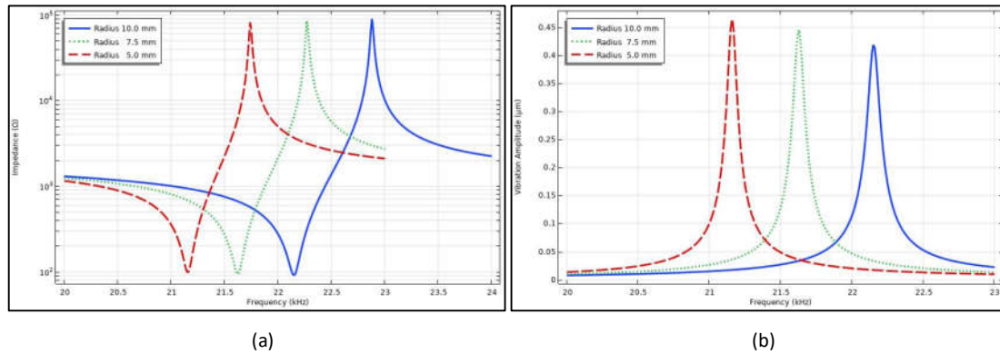
Figure 10 Simulation results of the Model-3 transducer (a) electrical impedance and (b) vibration amplitude with a 10-mm (solid blue line), 7.5-mm (dotted green line), and 5-mm (red dash line) fillet radius on a 15 kN prestressed bolt.
