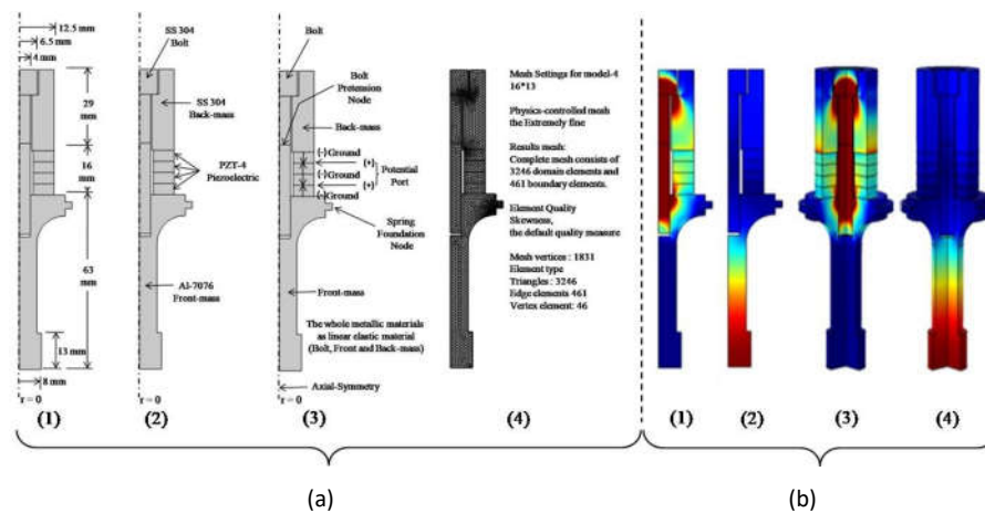
Figure 3 Stages of the piezoelectric ultrasonic transducer simulation process using the finite element method (a) pre-processing and (b) post-processing or optimization with visualization in 2D or 3D.
