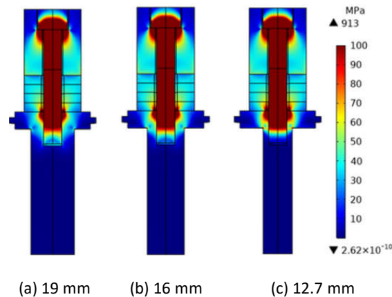
Figure 7 Simulation results of the stress distribution of the transducer with variations in the diameter of the horn at a bolt prestress value of 15 kN.
