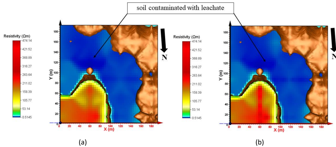
Figure 9 Resistivity image at ground level (a) 30 m, and (b) 33.8 m deep.
