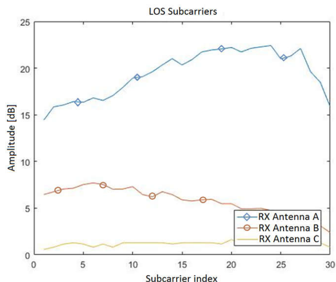
Figure 3 The strength curves of the three antennas.
