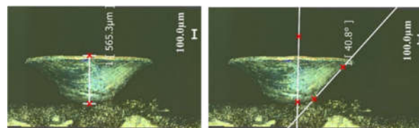
Figure 6 Figure lines for springback measurement.
