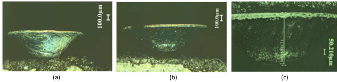
Figure 5 Micro cups under a digital microscope: (a) specimen 1 with drawing depth at 600 \mu\text{m} , (b) specimen 2 with drawing depth at 650 \mu\text{m} , and (c) specimen 3 with drawing depth at 550 \mu\text{m} .
