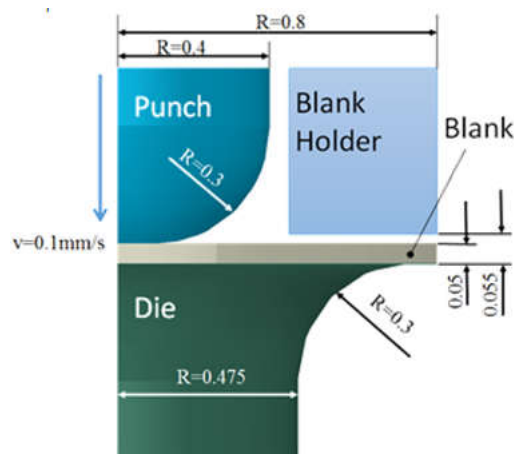
Figure 3 Schematic diagram of the MDD operation.
