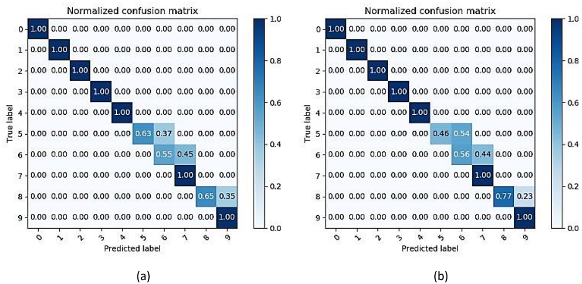
Figure 4 Confusion matrix modeling results with (a) RBF and (b) sigmoid kernels.
