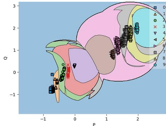
Figure 5 Normalized decision region modeling result with RBF kernel.
