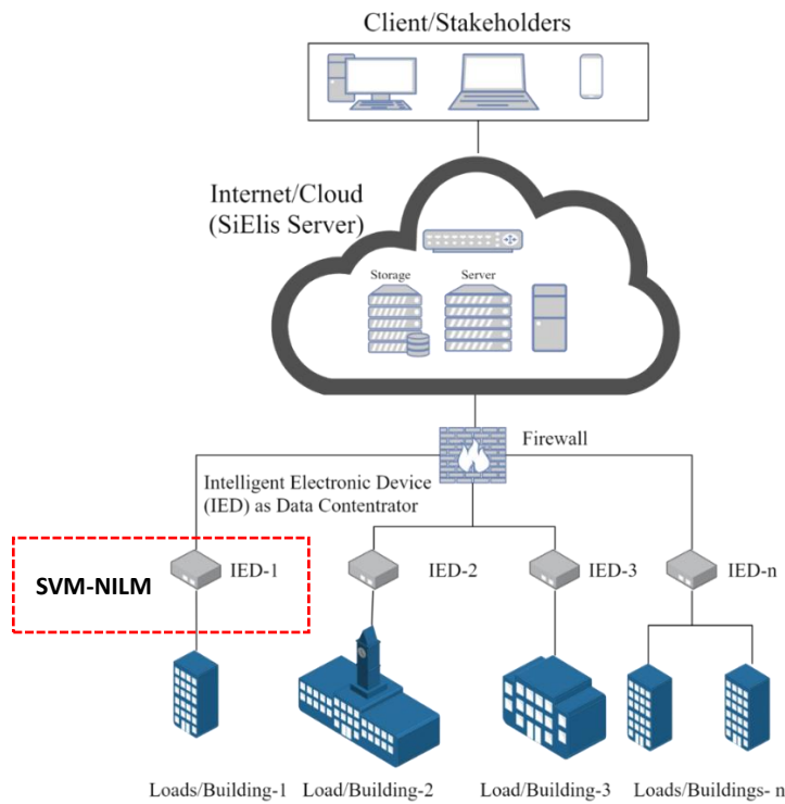
Figure 1 SiElis – Electricity Information System Concept.
