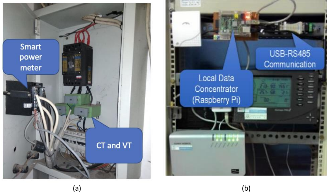
Figure 2 (a) IED - CT, VT sensor & smart power meter; (b) IED – data concentrator.
