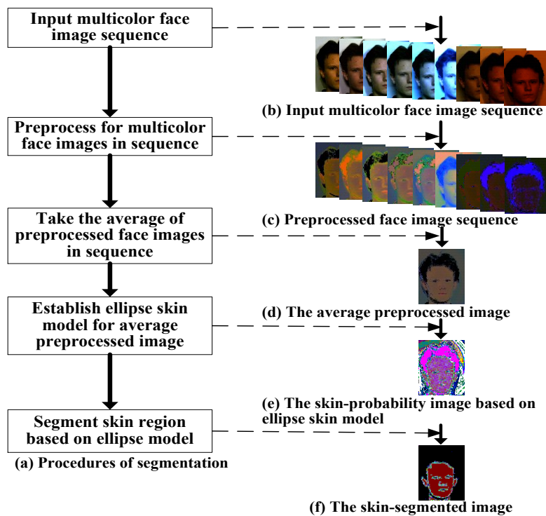
Figure 1 Procedure of segmentation and the acquired images.
