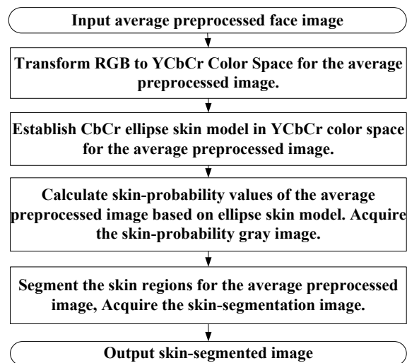
Figure 2 Procedures of skin segmentation
