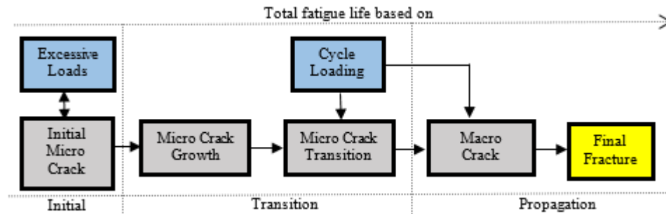
Figure 1 Description of the fatigue deterioration process in bridges.
