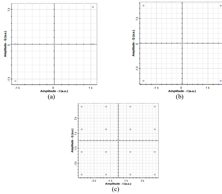
Figure 8 Constellation diagrams of RS 64 coded MIMO-based CO-OFDM FSO link for moderate turbulent environment at L = 5 km for (a) BPSK (b) QPSK and (c) 16-QAM.
