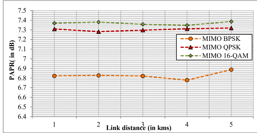
Figure 4 PAPR versus FSO link length for modulation schemes (BPSK, QPSK and 16-QAM) in a MIMO-based CO-OFDM FSO communication link using RS 64.
