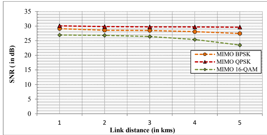
Figure 6 SNR with FSO link length for modulation schemes (BPSK, QPSK and 16-QAM) in a MIMO-based CO-OFDM FSO communication link using RS 64.
