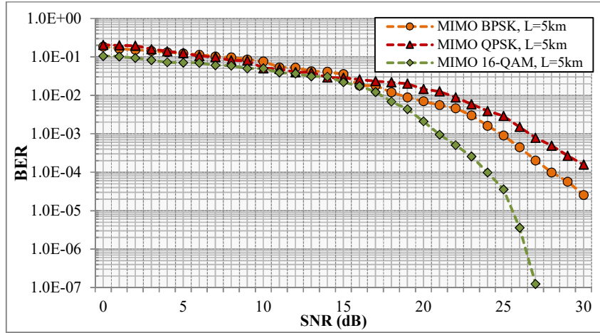
Figure 7 BER performance of BPSK, QPSK and 16-QAM modulated MIMO-based CO-OFDM FSO links using RS 64.
