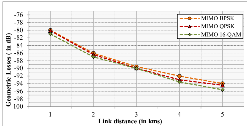
Figure 5 Geometric losses with FSO link length for modulation schemes (BPSK, QPSK and 16-QAM) in a MIMO-based CO-OFDM FSO communication link using RS 64.
