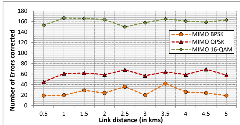
Figure 3 Errors corrected versus FSO link length for modulation schemes (BPSK, QPSK and 16-QAM) in a MIMO-based CO-OFDM FSO communication link using RS 64.
