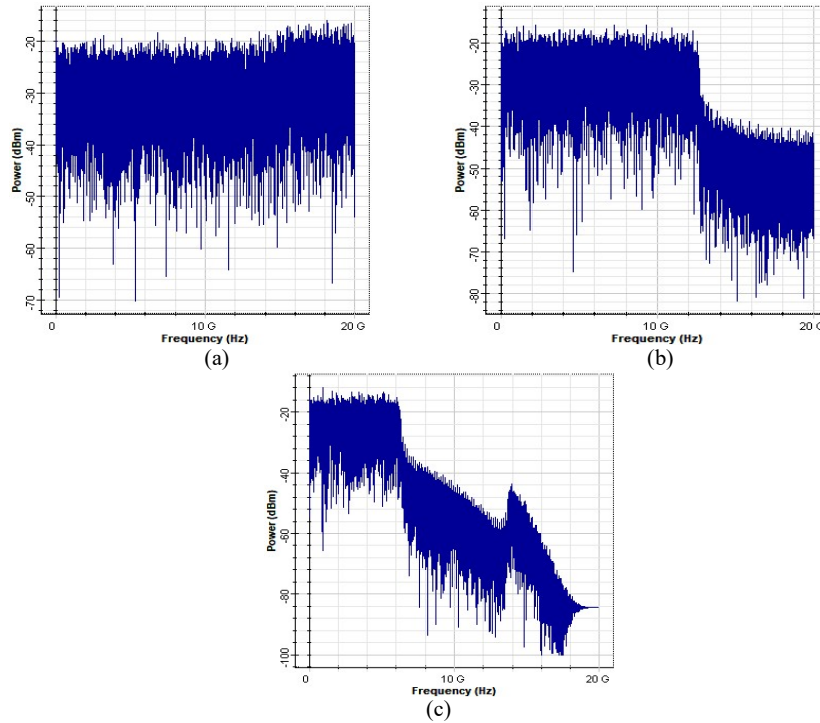
Figure 9 Spectrum analysis of proposed link after OFDM demodulation for (a) BPSK (b) QPSK and (c) 16-QAM.
