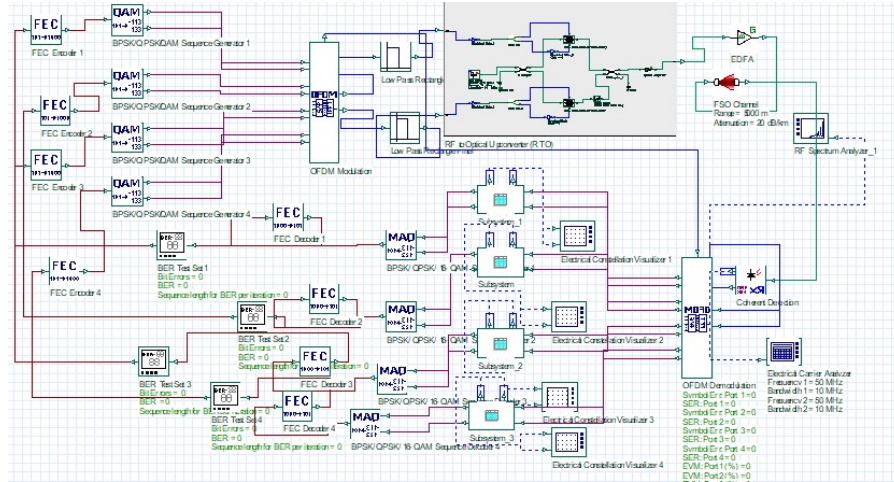
Figure 2 Simulation design of RS coded MIMO-based CO-OFDM FSO communication link using modulations schemes (BPSK, QPSK and 16-QAM) in Optisystem Simulator 16.1.
