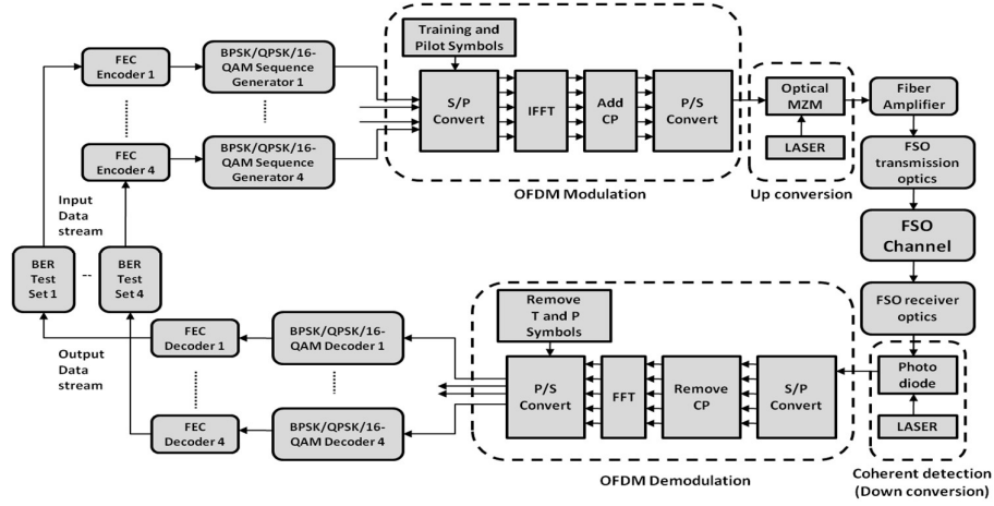
Figure 1 Proposed schematic comprising of transmitter and receiver of an RS coded MIMO-based CO-OFDM FSO communication link using modulation schemes (BPSK, QPSK and 16-QAM).
