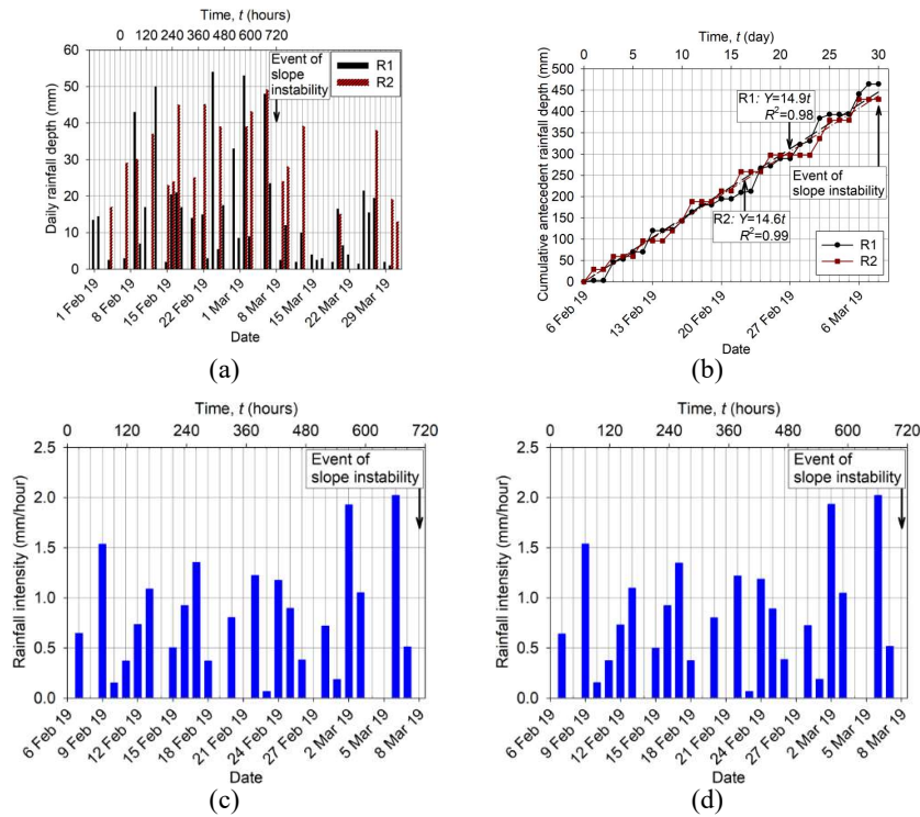
Figure 4 (a) Daily rainfall depth vs. time data, (b) cumulative antecedent rainfall depth, (c) interpolated rainfall intensity vs. time for slope no. 2, (d) interpolated rainfall intensity vs. time for slope no. 6.
