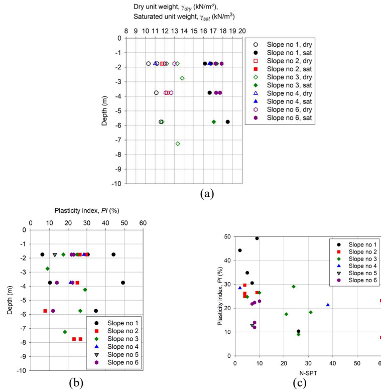
Figure 5 Soil properties obtained in June 2019: (a) variation of unit weight, \gamma with depth, (b) variation of plasticity index (PI) with depth, (c) PI vs. N-SPT (Data from [25]).
