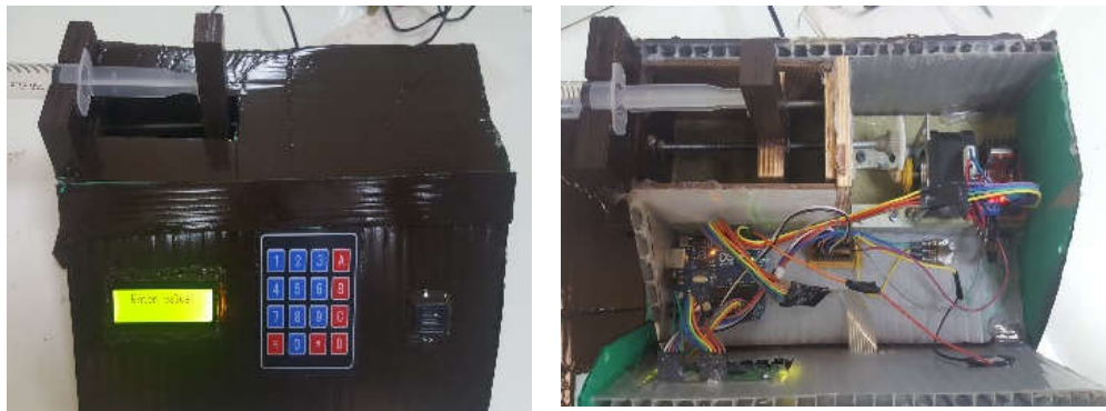
Figure 17 The complete implemented syringe pump.
