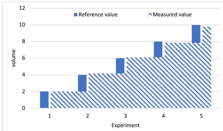
Figure 22 Measured error at of 100 ml/h speed.
