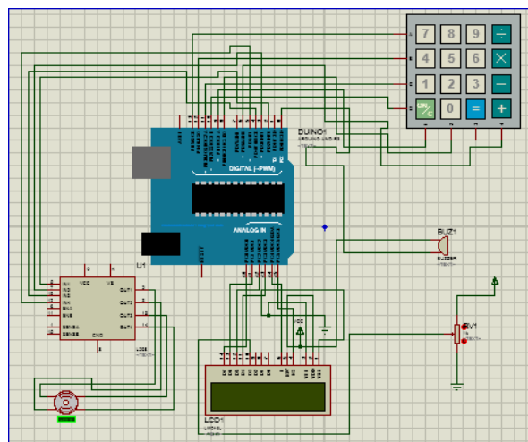
Figure 2 Proposed system circuit simulation.
