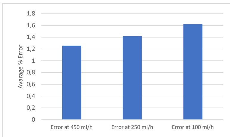
Figure 24 Average error percentages for the three speeds.
