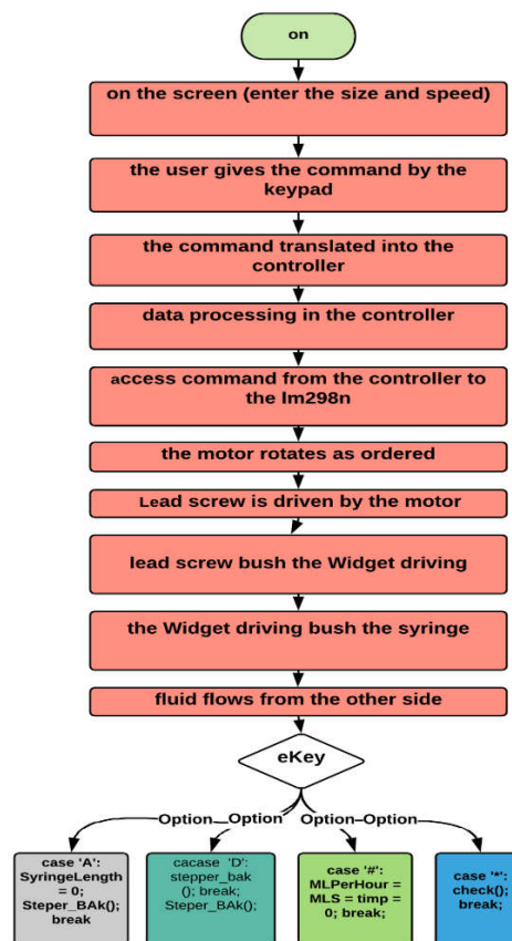
Figure 19 Machine operation mechanism.
