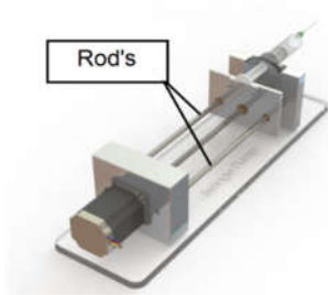
Figure 9 The rods.
