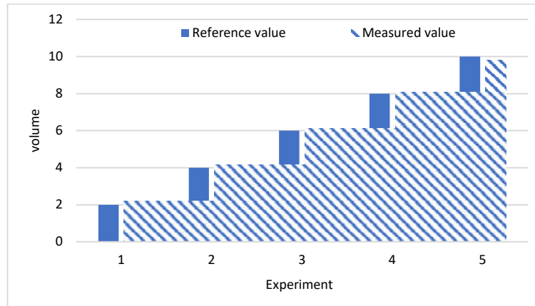
Figure 21 Measured error at 250 ml/h speed.
