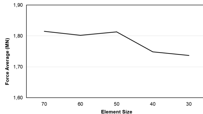
Figure 5 Grid independency.
