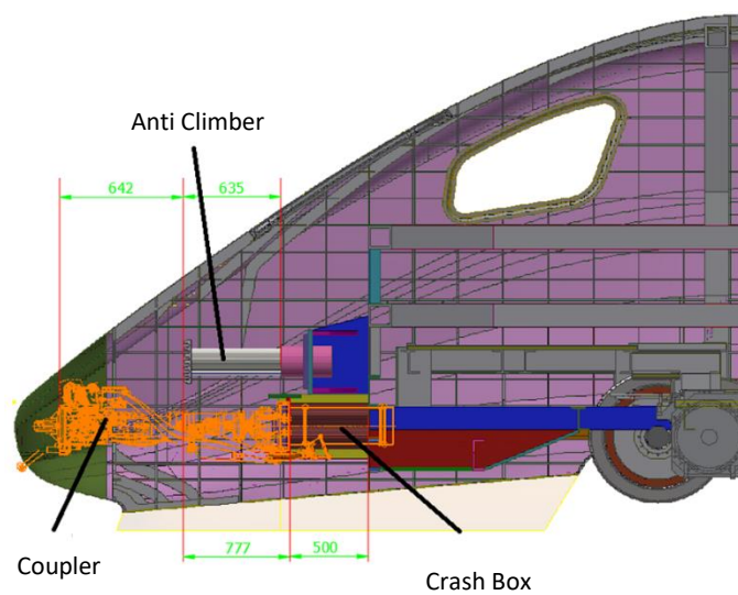
Figure 1 CEM design of the high-speed train.
