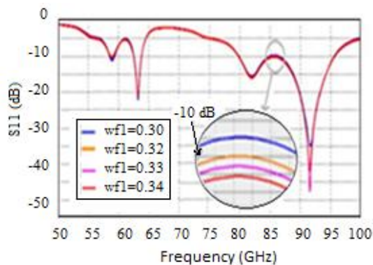
Figure 9 Reflection coefficient for the first method.
