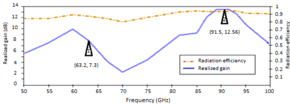
Figure 12 Realized gain and radiation efficiency.
