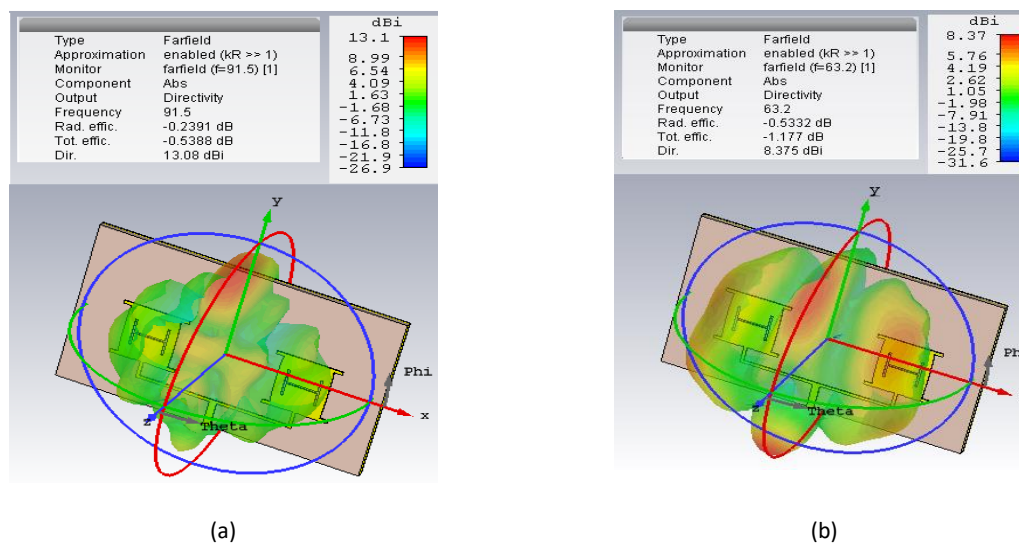
Figure 14 3D directivity radiation at: (a) 63.2 GHz, (b) 91.5 GHz.
