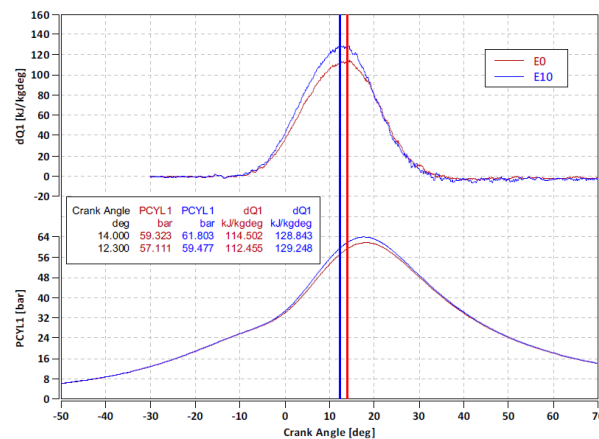
Figure 4 Heat release rate comparison for E0 and E10 at high speeds.
