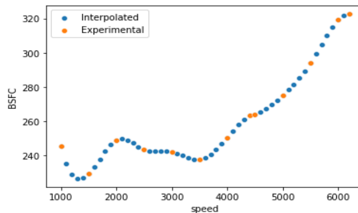
Figure 7 Interpolated engine performance data to conduct synthetic data generation.
