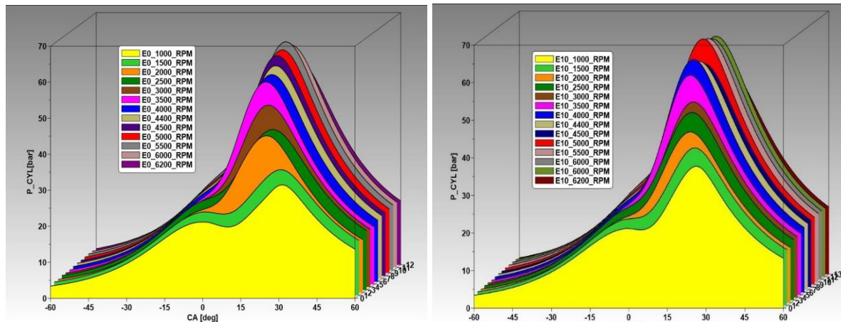
Figure 2 Waterfall diagram for P - \theta of the averaged-out data for E0 and E10 at all speeds.
