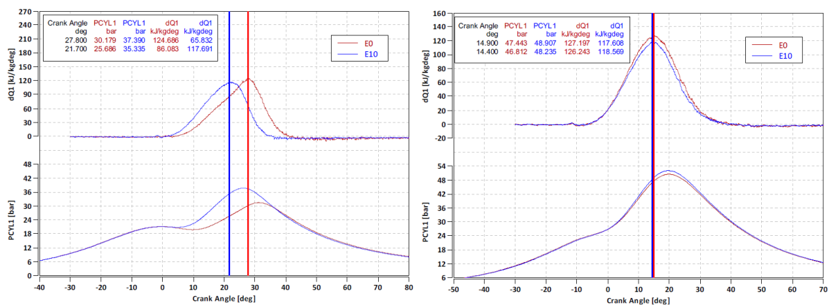
Figure 3 Heat release rate comparison for E0 and E10 at low and medium speed.
