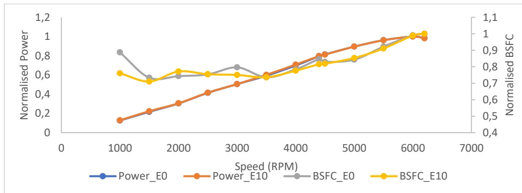
Figure 5 Power and BSFC comparison of averaged-out data for the E0 and E10 fuels.
