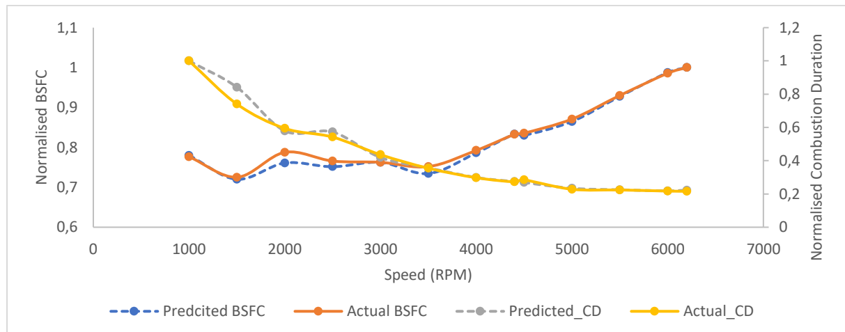
Figure 9 Predicted vs actual interpretation of engine BSFC and combustion duration for E15 data.
