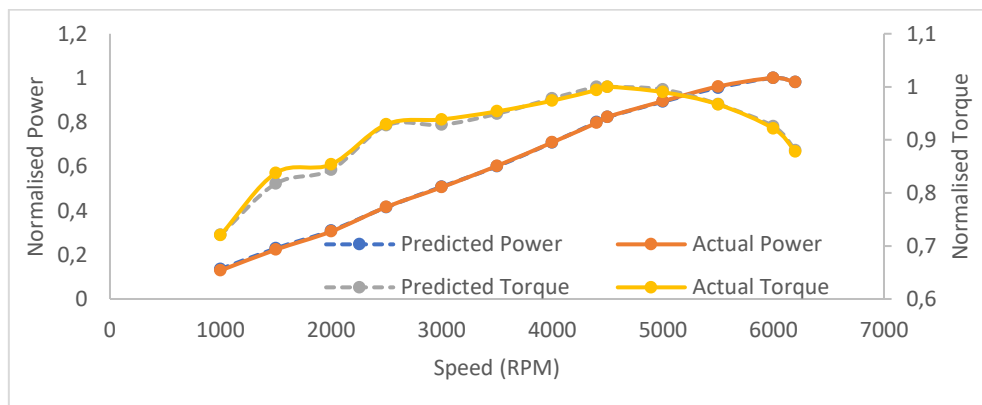
Figure 8 Predicted vs actual interpretation of engine power and torque for E15 data.
