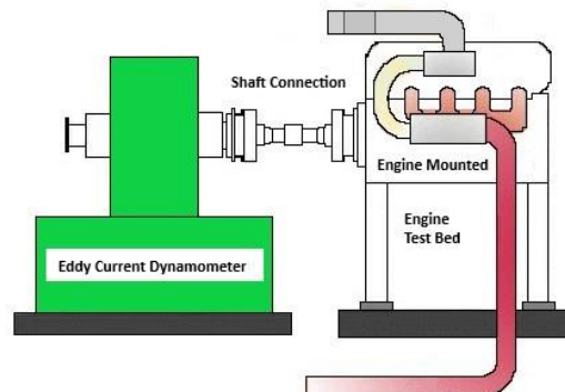
Figure 1 Schematics of eddy current dynamometer with engine mounted for testing.
