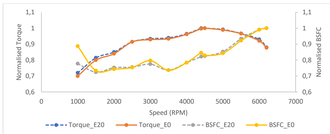
Figure 10 Predicted E20 vs actual E0 interpretation of engine power and torque.
