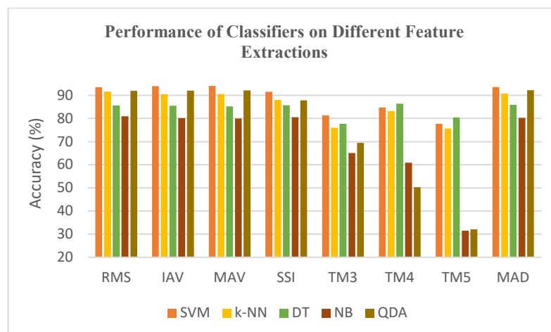
Figure 11 Classifier performance on different feature extractions
