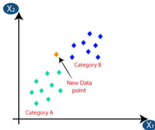
Figure 4 New data points based on k -NN neighbours [27].
