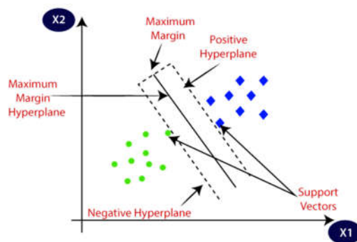
Figure 3 An example of an SVM decision boundary [27].
