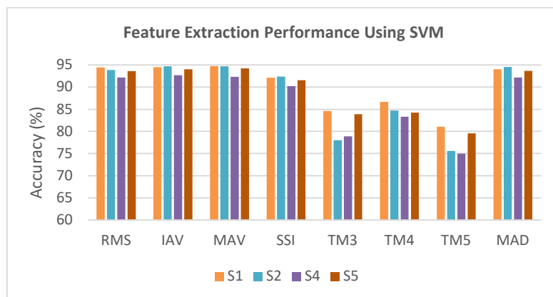
Figure 6 Feature extraction performance using SVM.
