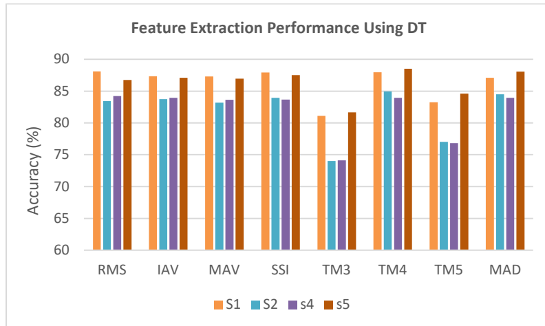
Figure 8 Feature extraction performance using DT.
