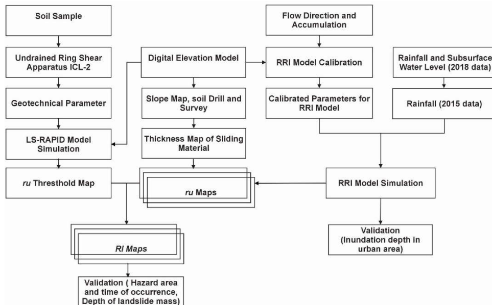
Figure 5 Major steps for coupling an LS-RAPID model and an RRI model to produce a rainfall-induced risk index (RI) map ( ru = pore water pressure ratio, RI = risk index) (retraced following Ha, Sayama [53]).
