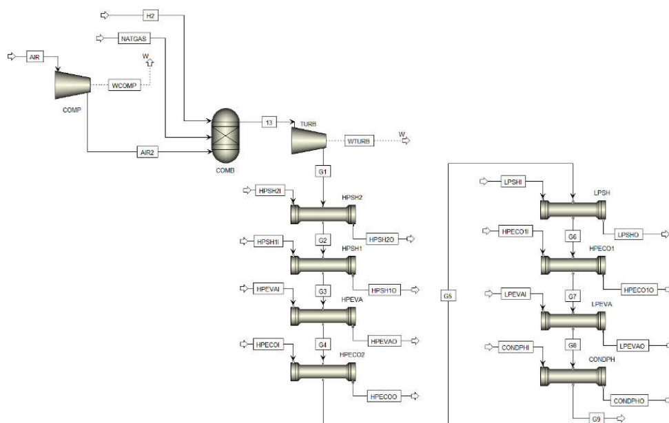
Figure 3 Detailed NGCC system.
