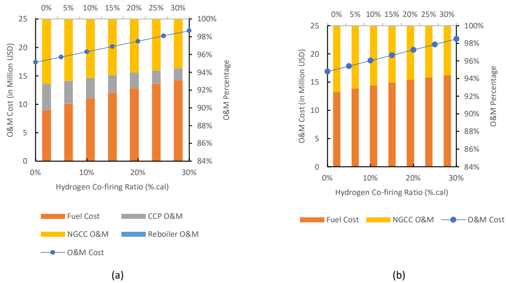
Figure 8 Operation and maintenance cost: (a) H2 Co-firing + CCP (b) H2 Co-firing.
