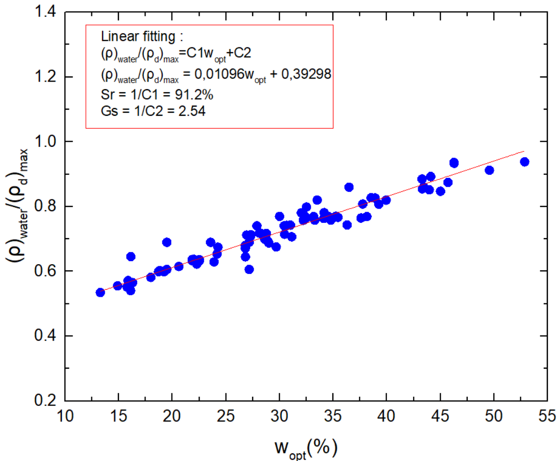
Figure 1 Relationship between (\rho_w)/(\rho_d)_{\max} and (w)_{\text{opt}} .
