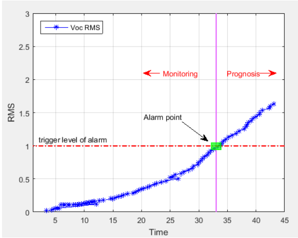
Figure 7 Online RMS evolution.
