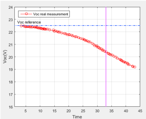
Figure 6 Real time monitoring of voltage Voc degradation.
