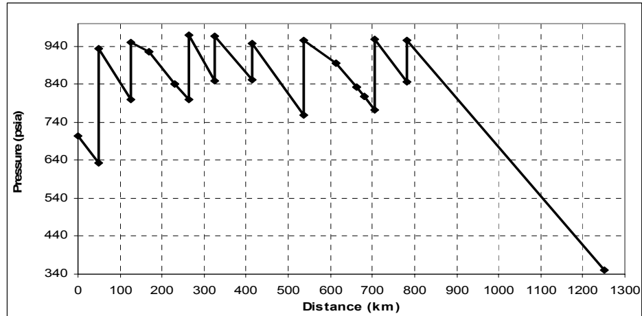
Figure 5 Pressure distribution for Optimum Result West Route .
