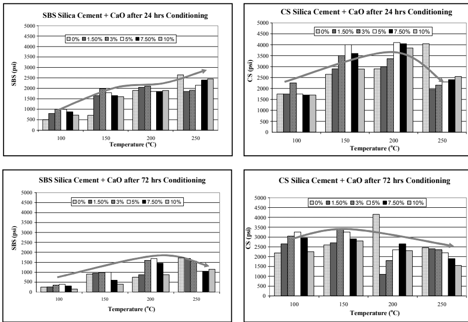
Figure 4.8 The Effect of CaO addition on Silica Cement.
