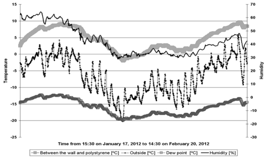
Figure 5 Graphical representation of the values obtained during the measurement series: humidity and temperature in the cavity between wall and insulation and temperature in the ambient surrounding of the building.
