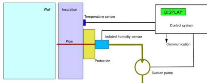
Figure 2 Schematic representation of the measurement equipment with its mutual connections.
