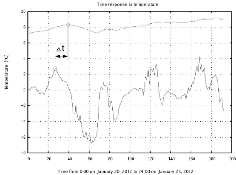
Figure 7 Graphical representation of the relationship between the temperature values in the space between wall and insulation and the ambient surrounding of the building.
