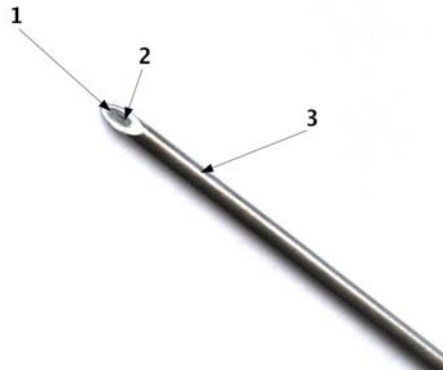
Figure 4 The pipe pierces through the panel of insulation material and transports the air sample to the chamber with the sensor. (1) Hole through the pipe, (2) polypropylene, (3) stainless steel.
