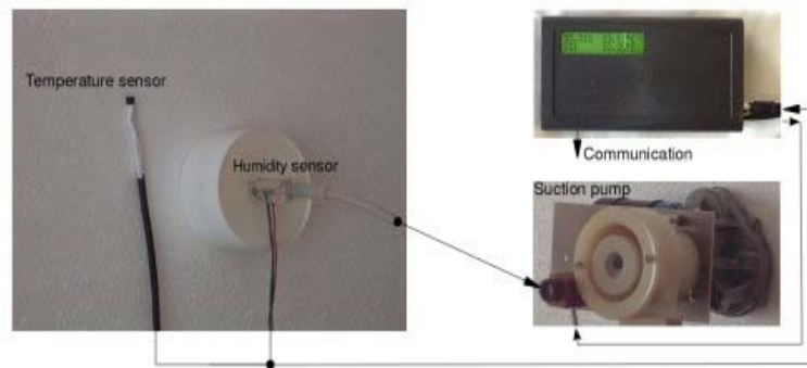
Figure 1 Measurement equipment used for testing the humidity and temperature levels in the space between wall and polystyrene insulation panels and also in the ambient surrounding outside of the building.
