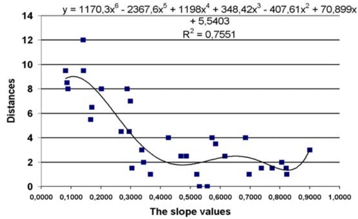
Figure 9 Graphical representation of the mutual relationship between slope sharpness and distance between the x-coordinates of the amplitudes of the temperature values ( x_i, y_i ) and the trend line of polynomial dependence given by Formula (2).
