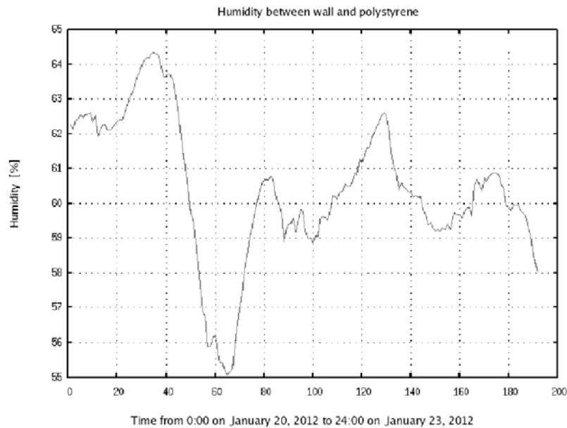
Figure 6 A graphical representation of humidity values in the cavity between wall and insulation material in detail.
