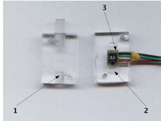
Figure 3 Sensor SHT15 with the chamber. (1) Upper part of the chamber, (2) lower part of the chamber, (3) sensor.
