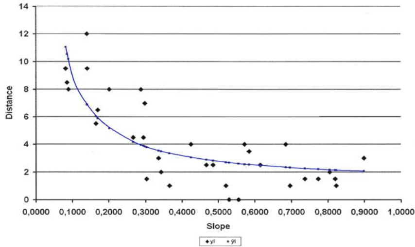
Figure 10 Graphical representation of the mutual relationship between slope sharpness and distance between the x -coordinates of the amplitudes of the temperature values ( x_j, y_j ) and the trend line of hyperbolic dependencies given by Formula (5) and passing through the points with coordinates (x_j, \hat{y}_j) .
