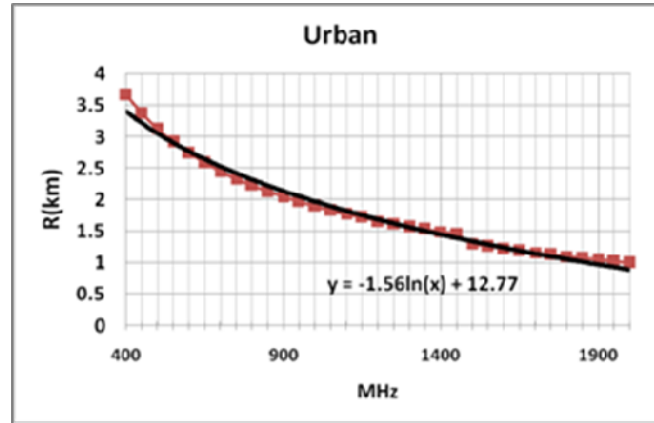
Figure 3 Frequency vs Range on band 400MHz -1900 MHz.
