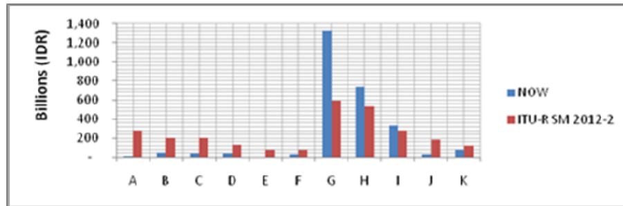
Figure 4 Spectrum fee paid by each operator.
