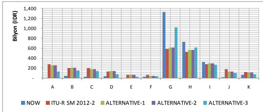
Figure 5 Comparison of calculation of spectrum fee.
