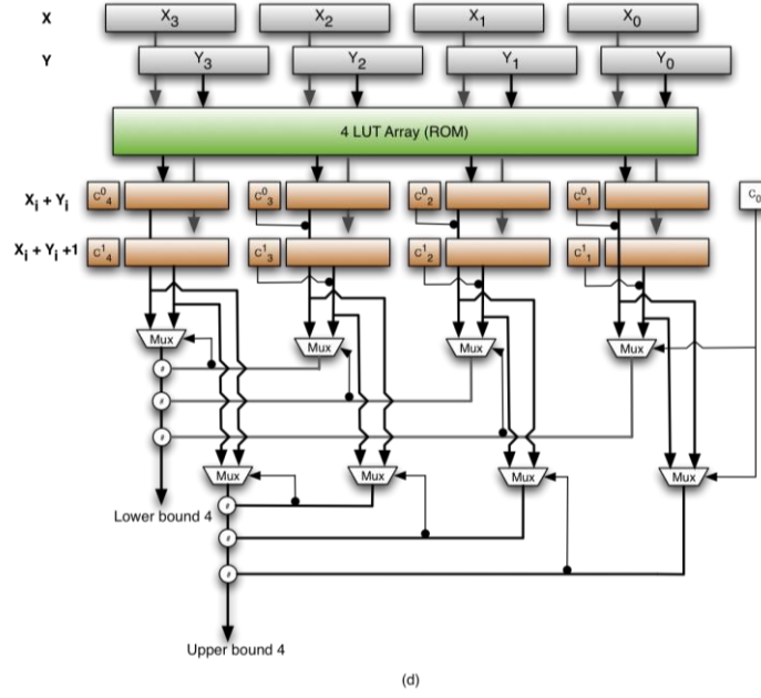
Figure 9 The MFIBVP adder schematic with n/k=4 ; (a to d) the fastest but least accurate to the slowest but most accurate computation.
