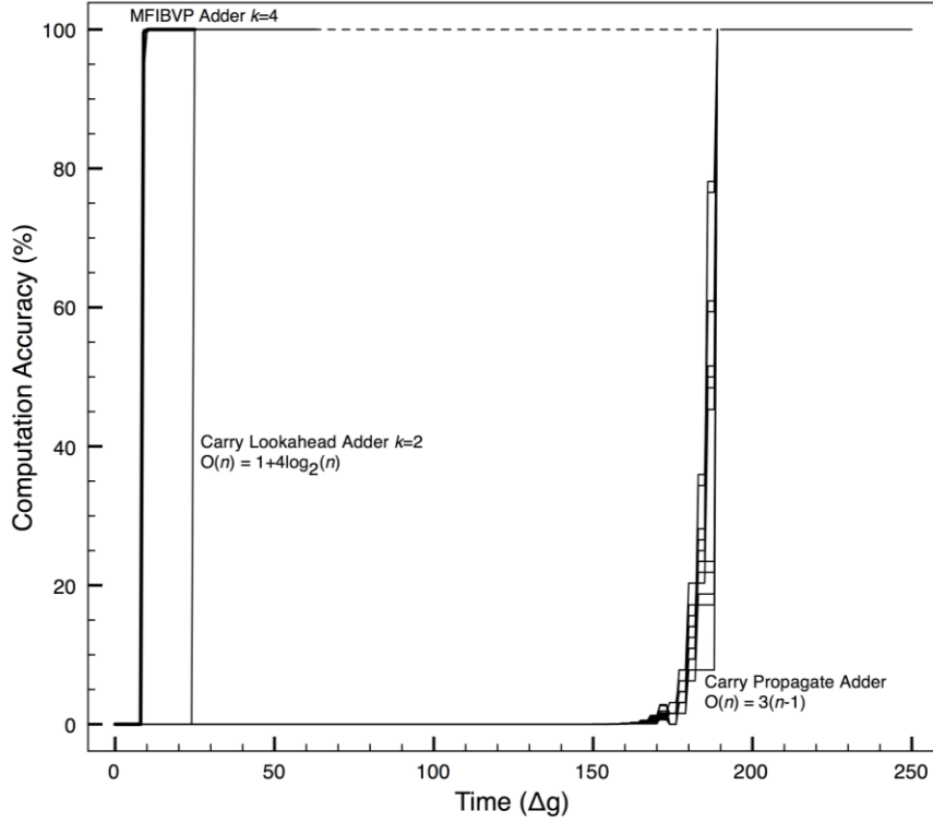
Figure 14 Performance comparison between the MFIBVP real-time adder vs Carry Look-ahead Adder and Carry Propagate Adder on 50 pairs of 64-bit random numbers.
