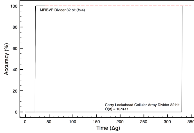
Figure 16 Performance comparison between the MFIBVP real-time divider vs Carry Look-ahead cellular array divider over 50 pairs of 32-bit random numbers.
