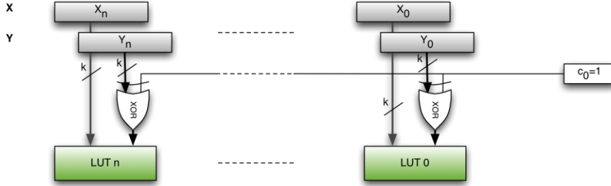
Figure 10 Additional XORs on the second operand will change the MFIBVP adder to a subtractor.
