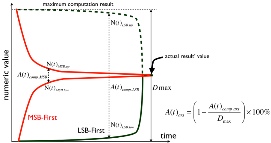
Figure 5 The interval bound concept of self-accuracy estimation by providing lower and upper bound value.
