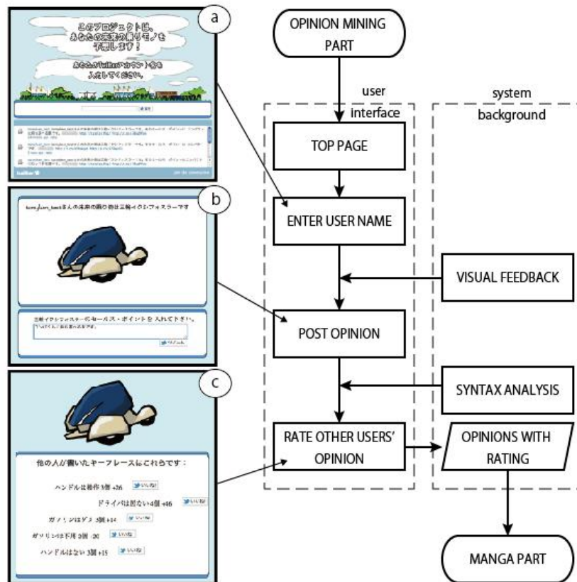
Figure 5 The opinion mining part(a) Login page (b) Idea entry page (c) Rating Page.
