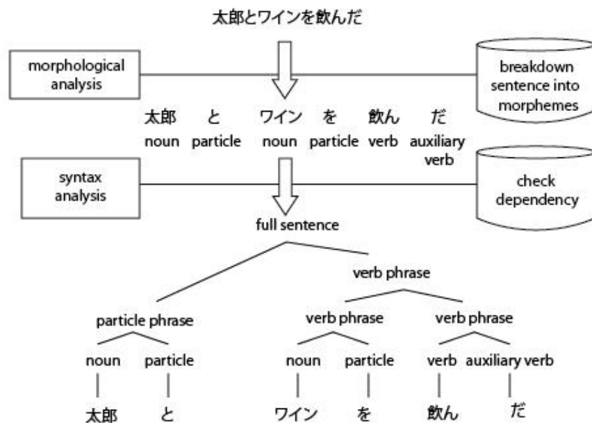
Figure 3 An example of morphological analysis and syntax analysis.
