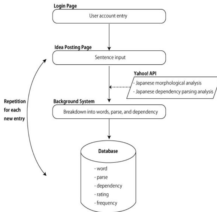
Figure 2 Morphological and Syntax analysis algorithm in our proposed system.
