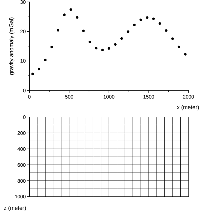
Figure 1 Illustration of the gravity anomaly data along a profile and associated 2D section with common x-axis. The subsurface domain on the x- and z-axis is discretized into grids representing 2D prisms.
