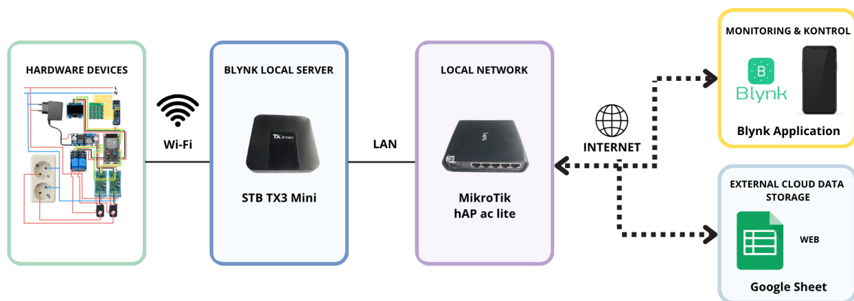
Figure 1. Block diagram of the hybrid-based IoT system
