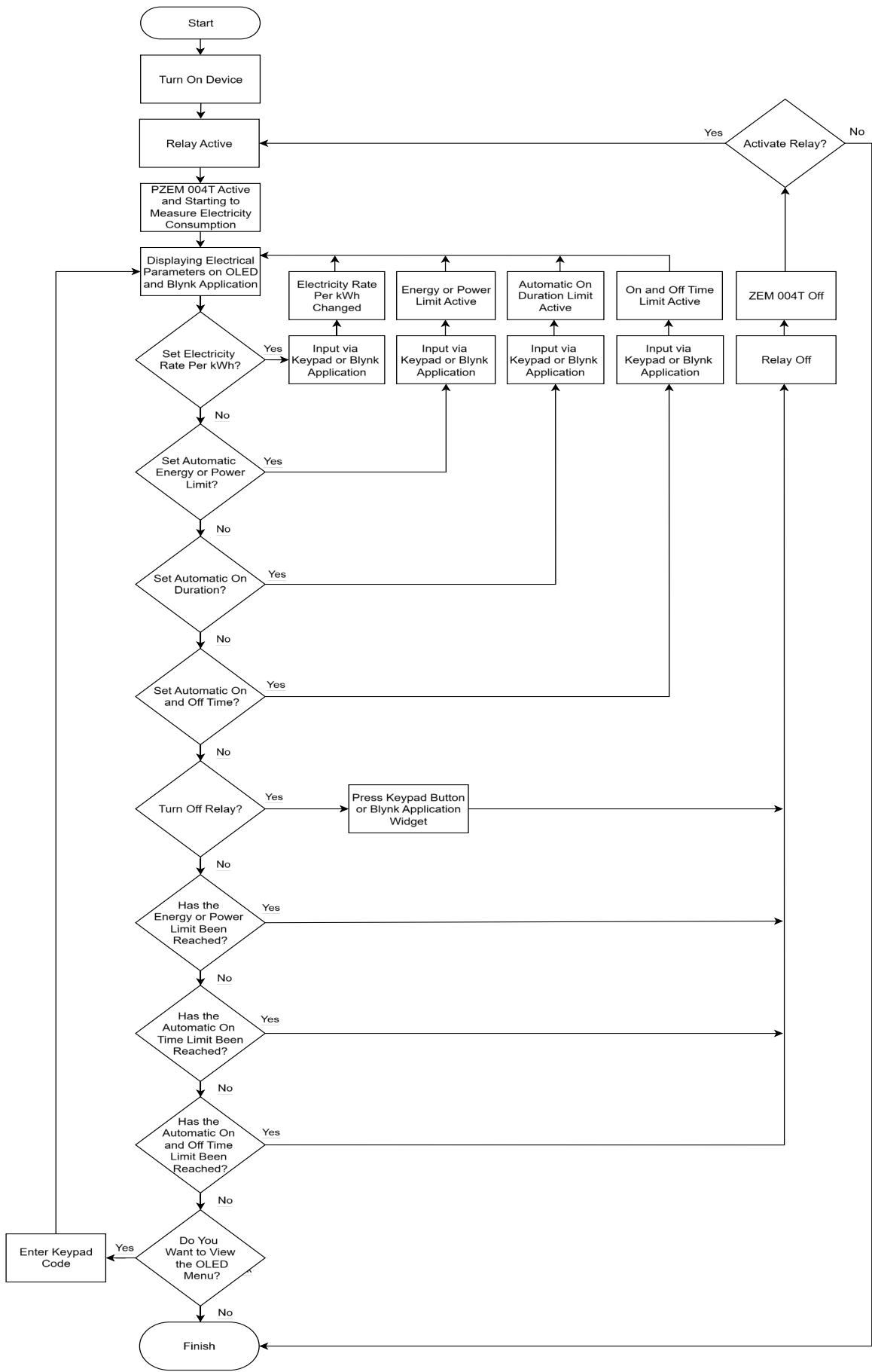
Figure 2. Working principle of the device
