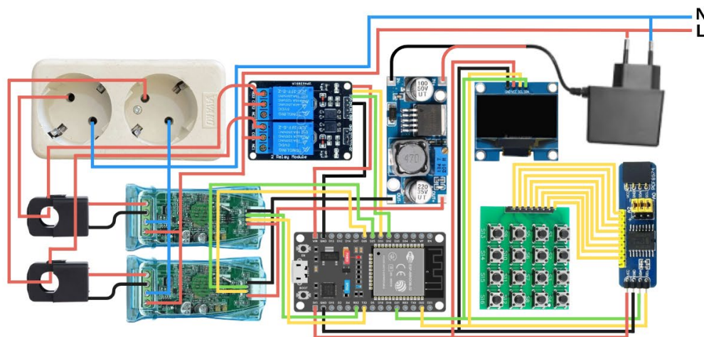
Figure 3. Wiring diagram of the designed device
