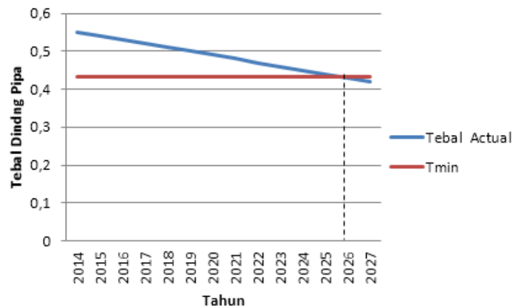
Gambar 5 Grafik Remaining Life Time pada Pipa Gas Lurus (Inlet Automatic Shutdown Valve KP-20 Ø 20")
