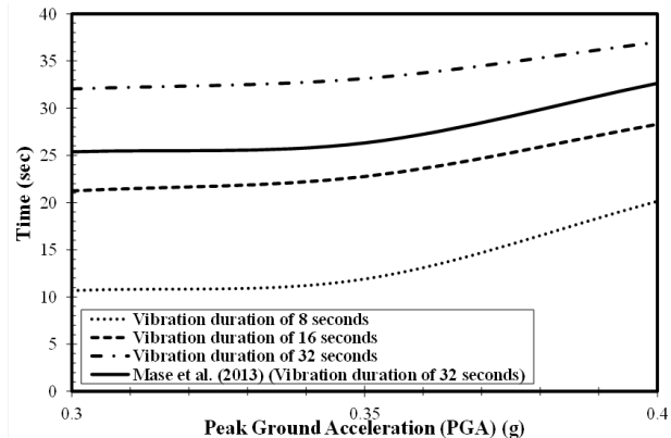
Figure 8. The variation in duration of liquefaction with Peak Ground Acceleration (PGA)
