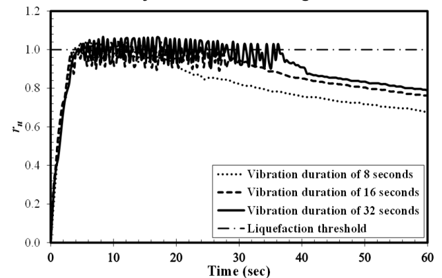
Figure 6. The ratio of pore water pressure vs time for dynamic load of 0.4 g
