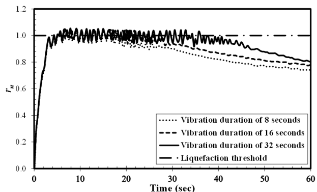
Figure 4. The ratio of pore water pressure vs time for dynamic load of 0.3 g
