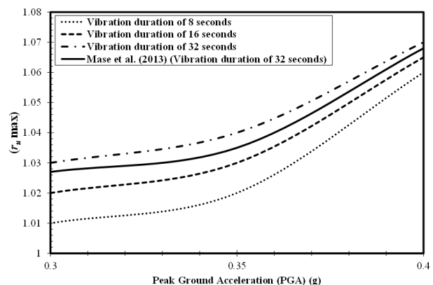
Figure 9. The variation in maximum excess pore water pressure ratio ( r_u max) with Peak Ground Acceleration (PGA)
