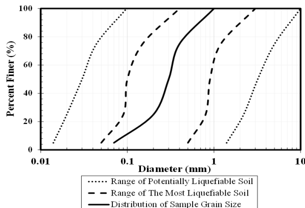
Figure 3. Comparison between grain size distribution and the grain size distribution proposed by Tsuchida (1970)
