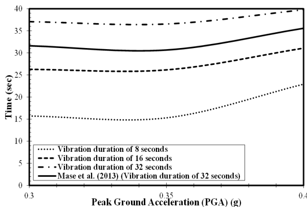
Figure 7. The variation in time to be dissipated liquefaction with Peak Ground Acceleration (PGA)
