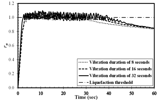
Figure 5. The ratio of pore water pressure vs time for dynamic load of 0.35 g
