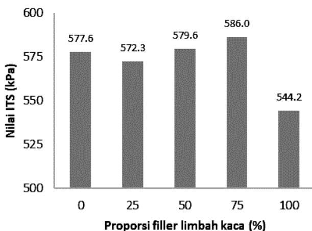
Gambar 9. Nilai ITS pada kadar aspal optimum
