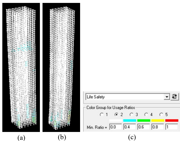
Figure 8. Final condition of 1.2 cs average model – el alamo: (a) X dir, (b) Y dir, (c) colour group
