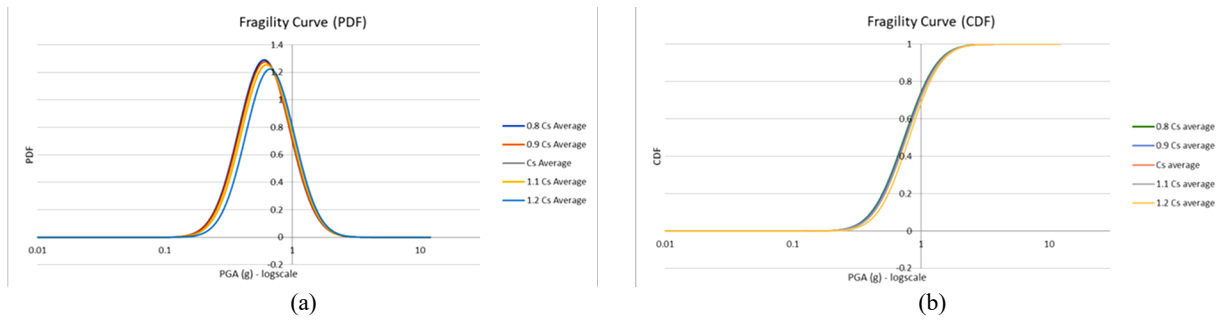
Figure 9. Fragility curve: (a) (PDF), (b) (CDF)
