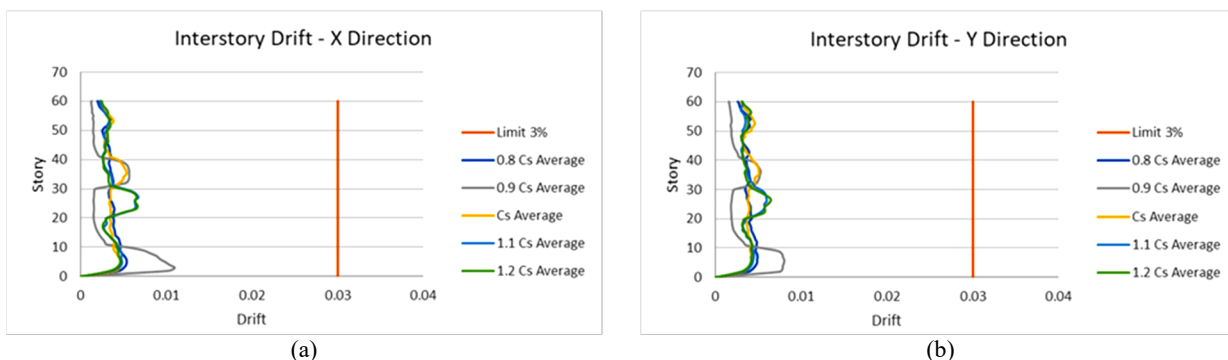
Figure 6. Inter-story Drift: (a) X Direction, (b) Y Direction
