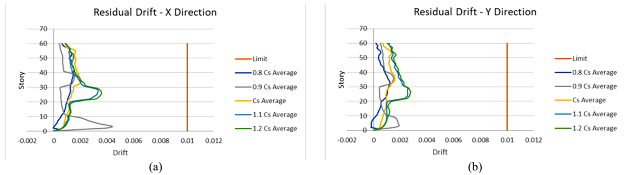
Figure 7. Residual drift: (a) X direction, (b) Y direction
