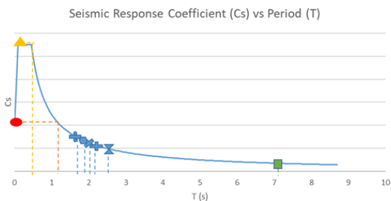
Figure 5. Illustration of seismic response coefficient
