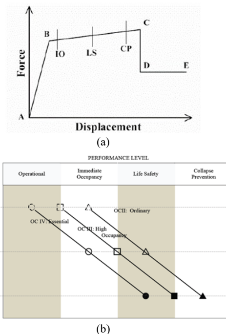
Figure 2. (a) Capacity curve ATC-40, (b) Performance Level
