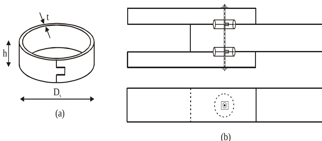
Figure 1. Flat split-ring (a) and split-ring connection (b)
