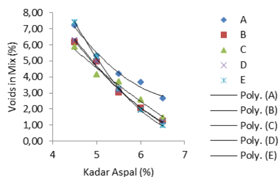
Gambar 6. Kadar aspal vs VIM
