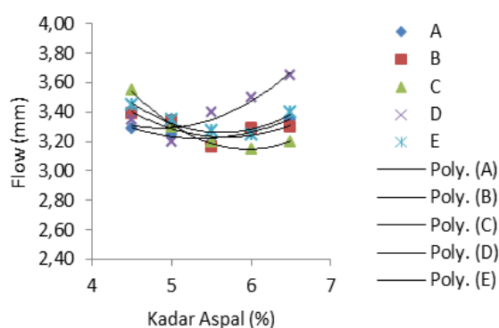
Gambar 4. Kadar aspal vs flow
