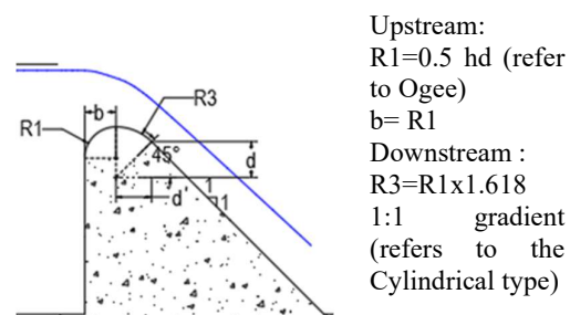
Figure 5. Geometry of ITB Golden Ratio type B (Annas Syaeful, 2025)
