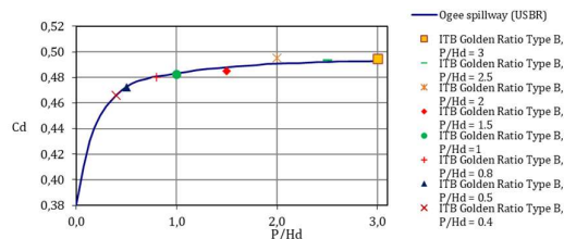
Figure 11. Discharge Coefficient ( C_d ) of ITB Golden Ratio type B
