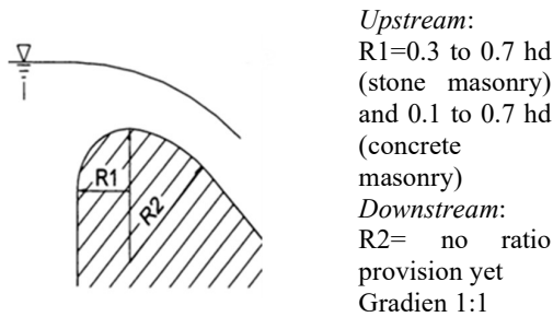
Figure 2. Geometry of the cylindrical crest (PU Dirjen SDA 2013)
