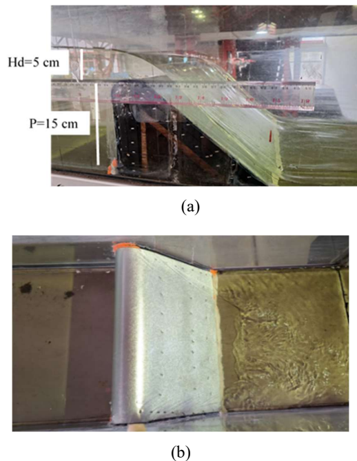
Figure 14. ITB Golden Ratio Spillway Type B Model with a 1:40 scale, up picture (a): side view, bottom picture(b): top view.
