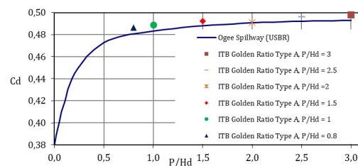
Figure 9. Design Discharge Coefficient ( C_d ) of ITB Golden Ratio type A
