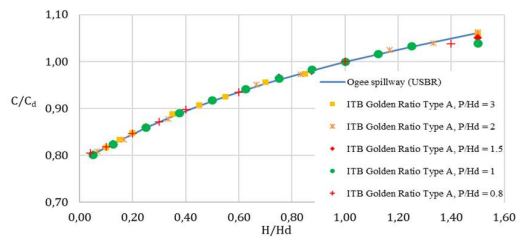
Figure 10. Correction Coefficient C/C_d of ITB Golden Ratio type A
