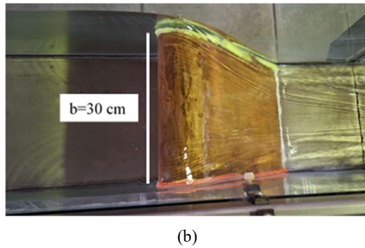
Figure 13. ITB Golden Ratio Spillway Type A Model with a 1:25 Scale, Up picture (a): side view, bottom picture (b): top view
