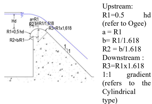
Figure 4. Geometry of ITB Golden Ratio type A (Annas Syaeful, 2025)
