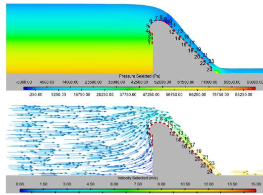
Figure 7. Velocity flow pressure profile on Spillway Golden Ratio type A
