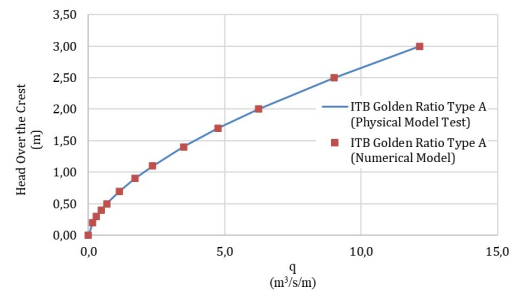
Figure 15. Comparison of ITB Golden Ratio Type A Spillway Discharge Curve (P/Hd=3, vertical upstream) from Physical Model Test and Numerical Model.
