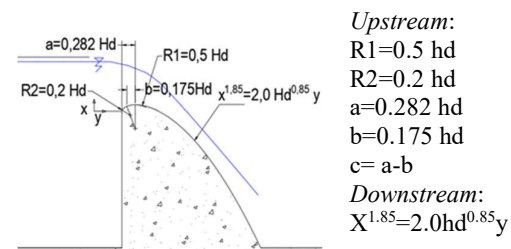
Figure 1. Geometry of ogee crest (PU Dirjen SDA, 2013)
