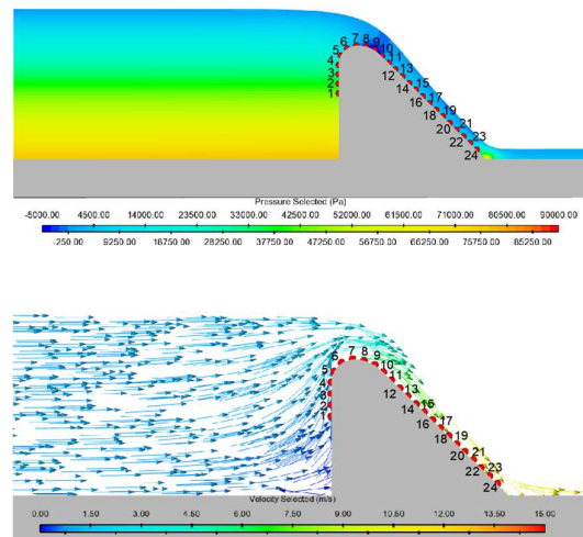
Figure 8. Velocity flow pressure profile on Spillway Golden Ratio type B
