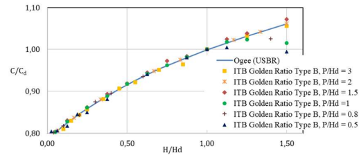
Figure 12. Correction Coefficient C/C_d of ITB Golden Ratio type B
