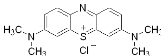
Gambar 1. Struktur zat methylene blue (Anonymous, 2009)
